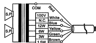
STANDARD CONNECTION
