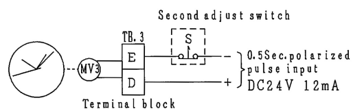
Wiring diagram
