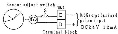
Wiring diagram
